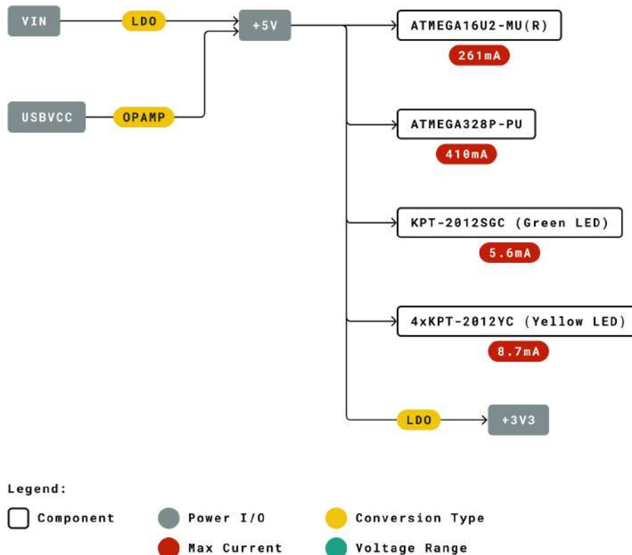
Power tree
