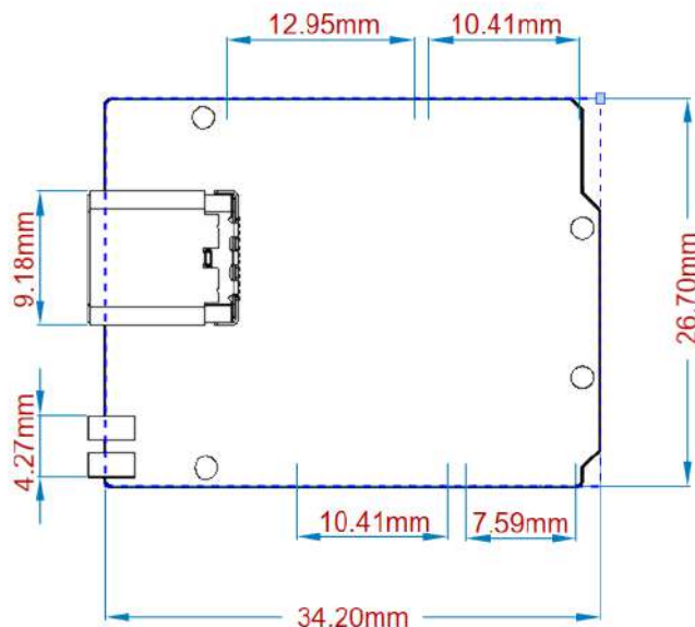
Board outline
