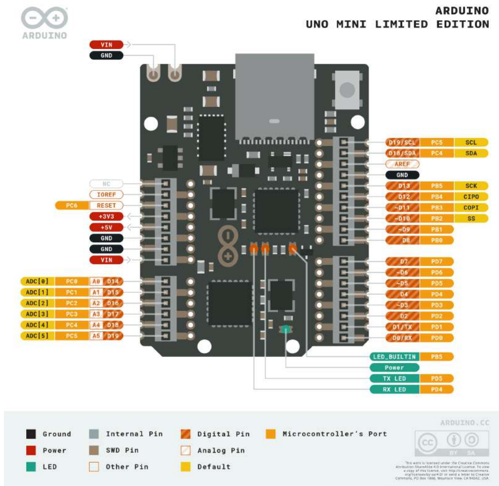
Pinout
